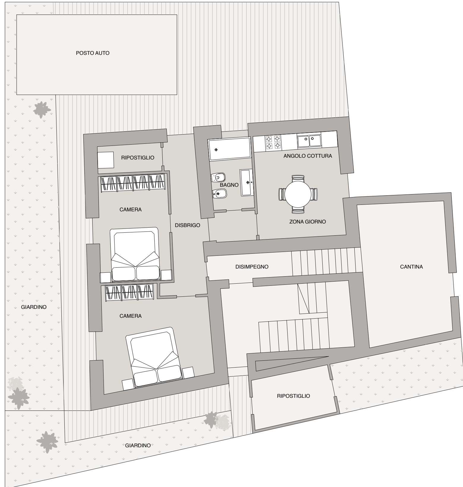
PIANO TERRA
